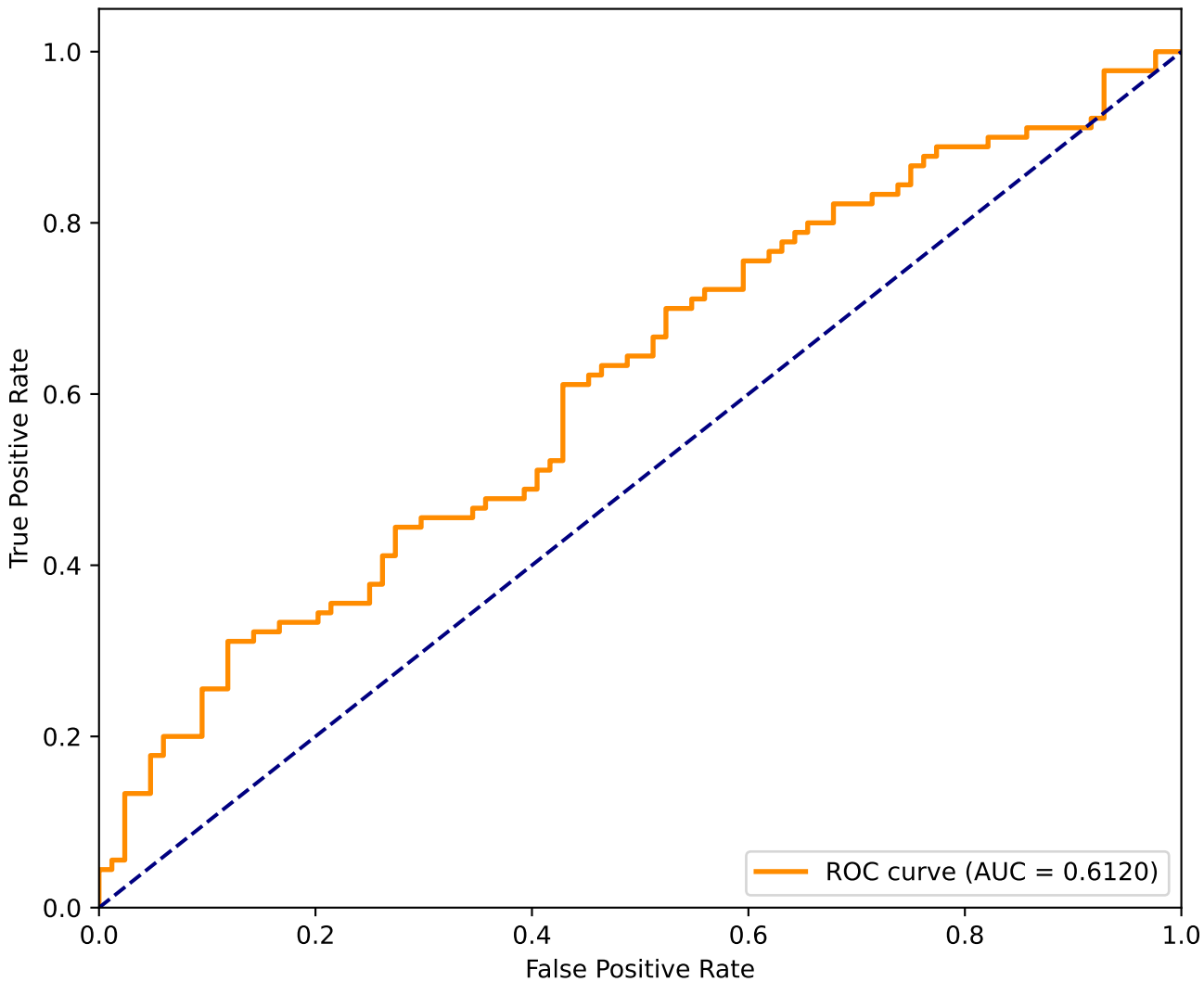
ROC Curve - MLP
